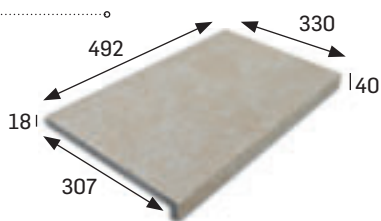
PELDAÑO RECTO 50 STRAIGHT STAIR-TREAD 50 [492x330x18 mm]
