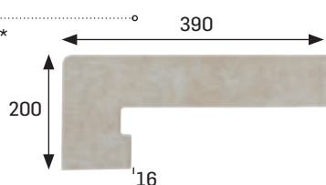
ZANQUÍN IZDA. RECTO STRAIGHT STRING LEFT SIDE * [390x80/200x100x16 mm]
